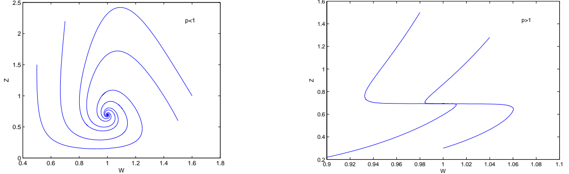
Figure 1: Solutions to System (44) are plotted in the phase plane (W, Z) for two different values of parameter p . The other coefficients are \gamma = 0.1 , \mu = 1 and f(x) = 2e^{-x} . We can see that the steady state is a focus for p < 1 (left) and a node for p > 1 (right).
